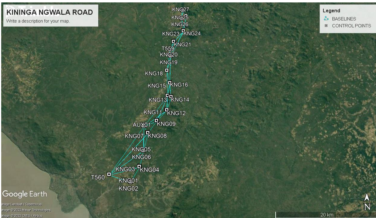
GPS Triangulation network
